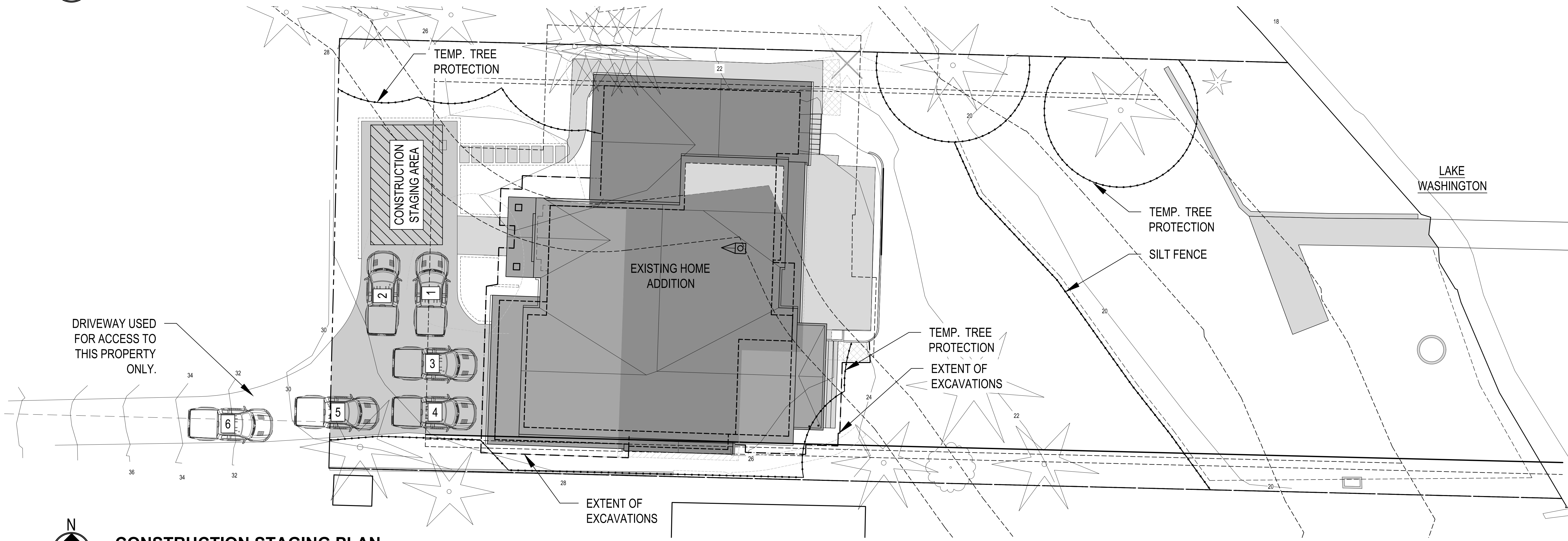
CONSTRUCTION STAGING PLAN SCALE: 1"=10'-0"
